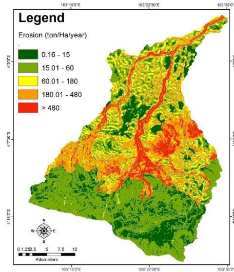
Figure 5. Distribution of Erosion at the Endikat Watershed
